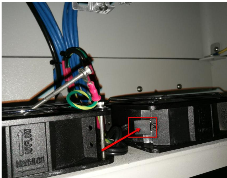
Figure 6 Cable assembly
